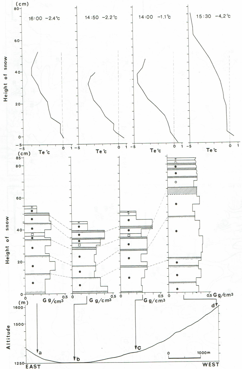
Fig. 6. Vertical profile of snow temperature (upper), stratigraphic diagrams of four snow layers (middle) along the cross section (lower) shown in Fig. 1(b). Units are ^{\circ}\text{C} for snow temperature ( T_e ), \text{g}/\text{cm}^3 for snow density ( G ).
